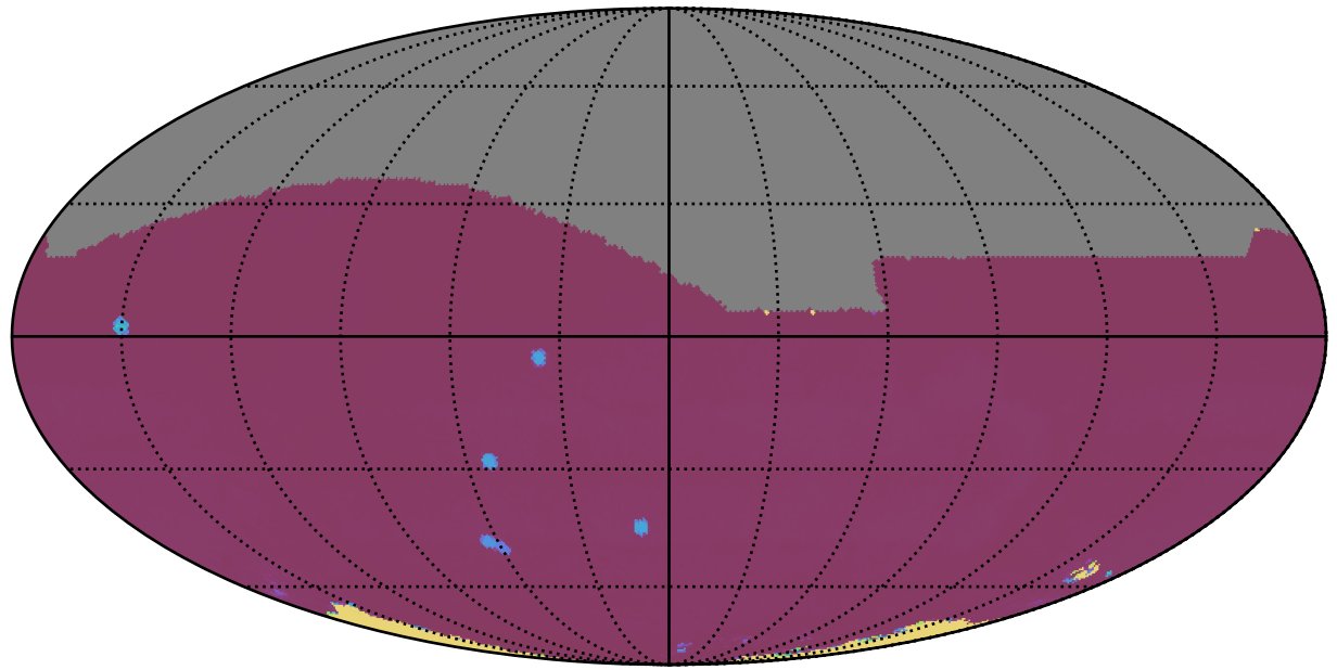
extra_ss_neo4_v3.4_10yrs All sky all bands: 75th Percentile Intranight Timespan
