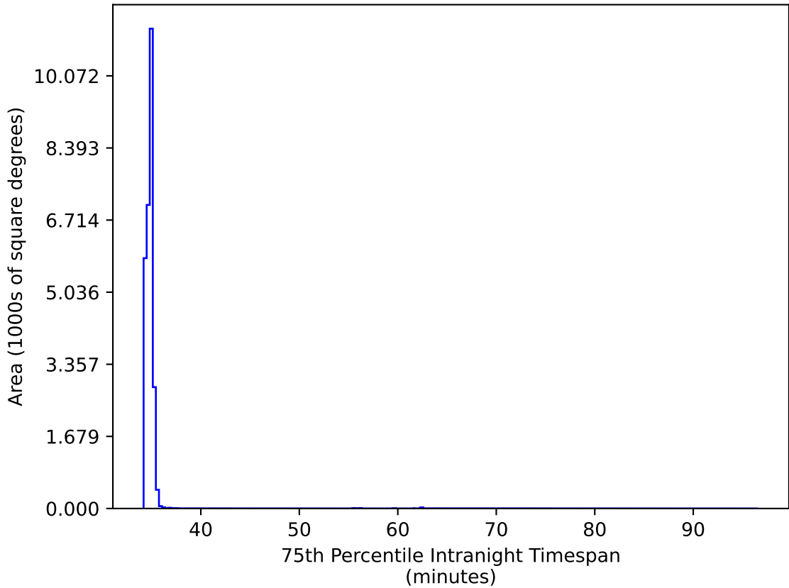
extra_ss_neo4_v3.4_10yrs All sky all bands: 75th Percentile Intranight Timespan
