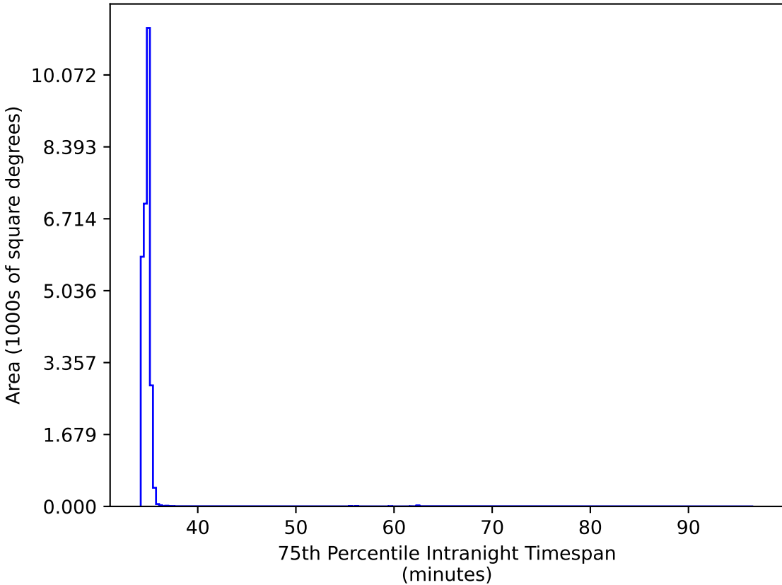
extra_ss_neo4_v3.4_10yrs All sky: 75th Percentile Intranight Timespan
