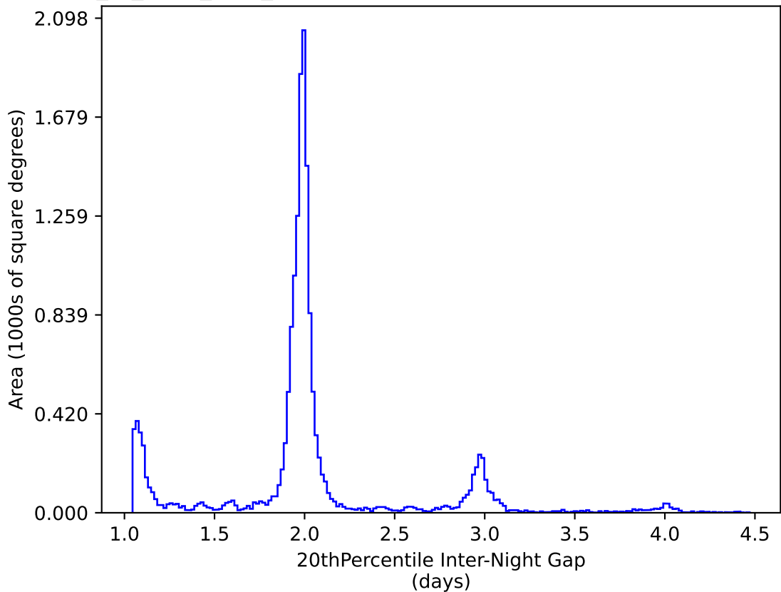
extra_ss_neo4_v3.4_10yrs WFD y band: 20thPercentile Inter-Night Gap
