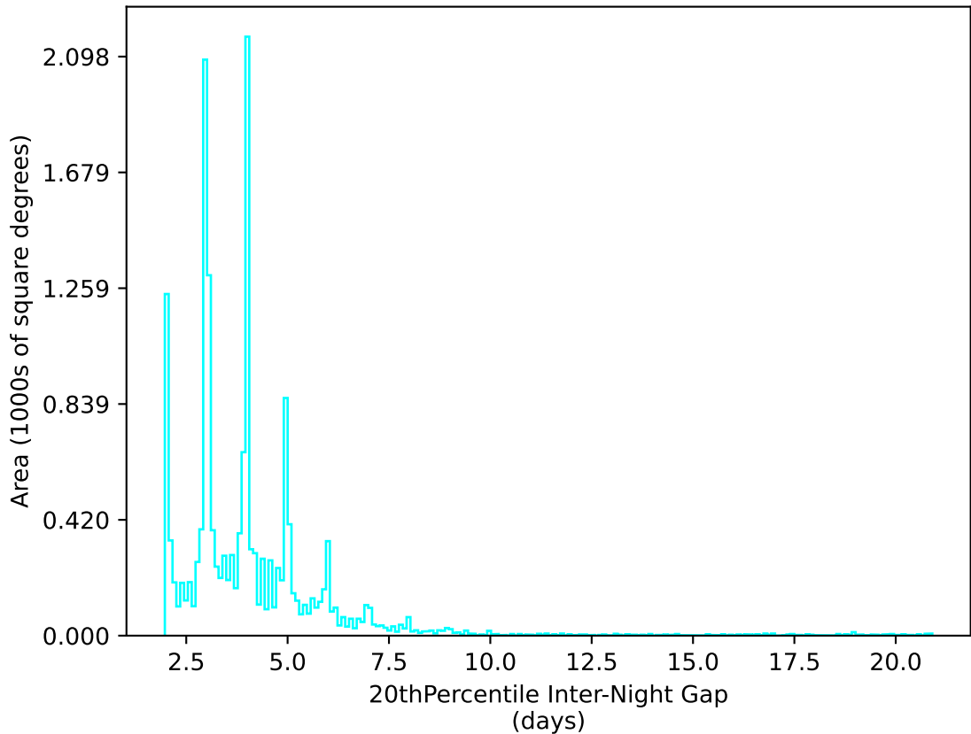
extra_ss_neo4_v3.4_10yrs WFD u band: 20thPercentile Inter-Night Gap
