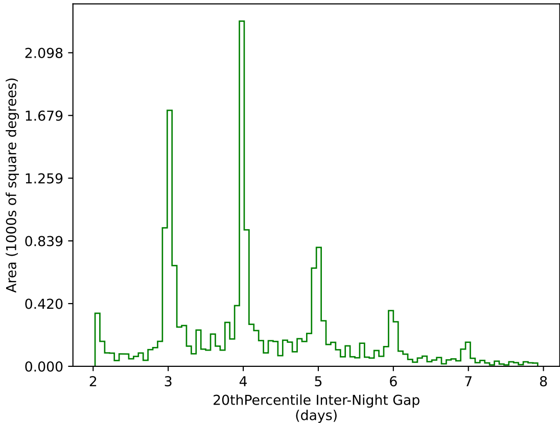
extra_ss_neo4_v3.4_10yrs WFD g band: 20thPercentile Inter-Night Gap
