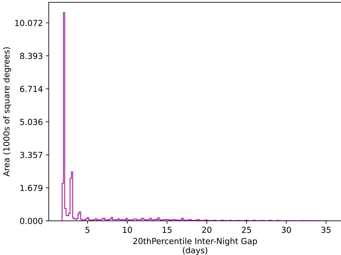
extra_ss_neo4_v3.4_10yrs All sky z band: 20thPercentile Inter-Night Gap
