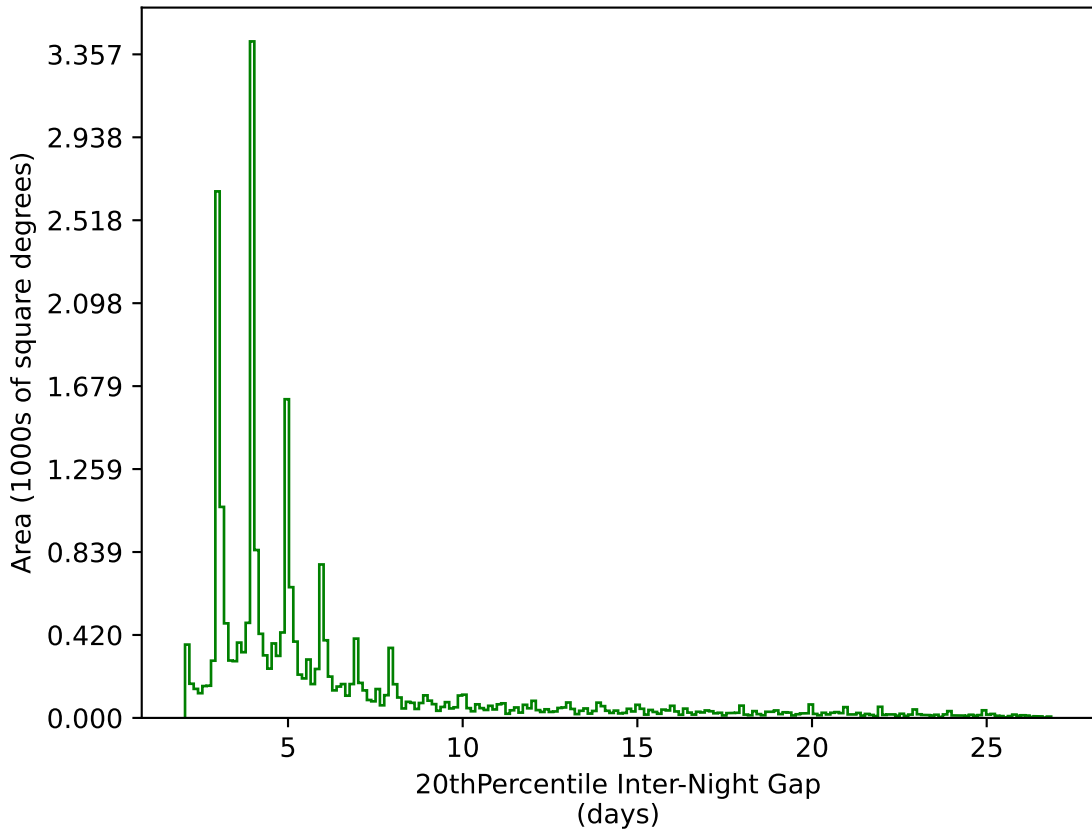
extra_ss_neo4_v3.4_10yrs All sky g band: 20thPercentile Inter-Night Gap
