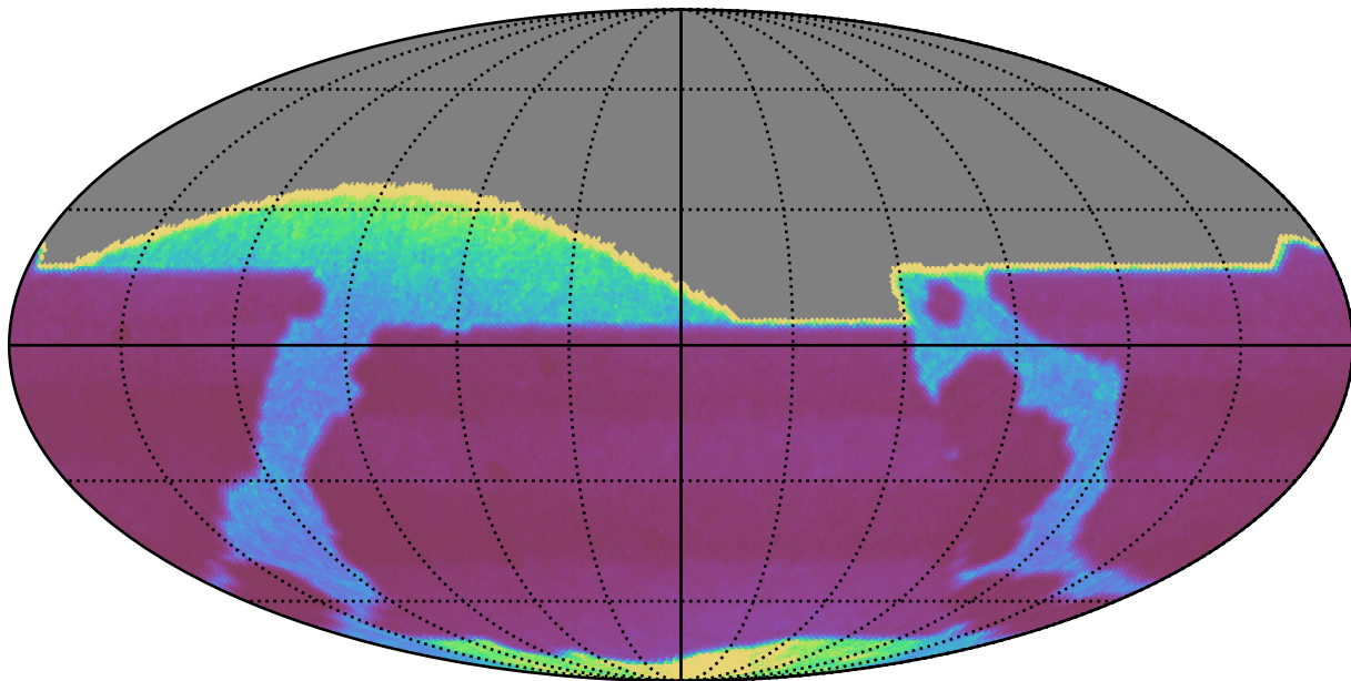
extra_ss_neo4_v3.4_10yrs : properMotion
