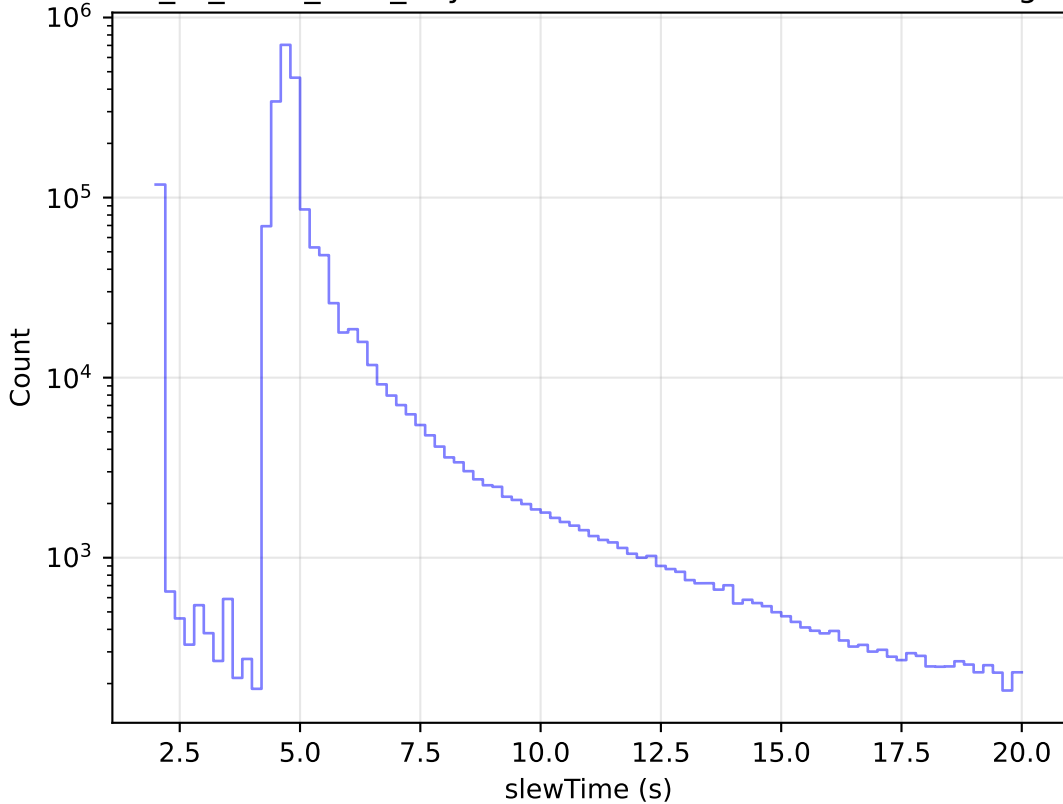
extra_ss_neo4_v3.4_10yrs All visits: Zoom Slew Time Histogram
