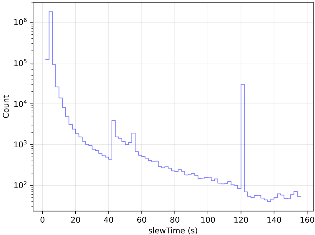
extra_ss_neo4_v3.4_10yrs All visits: Slew Time Histogram
