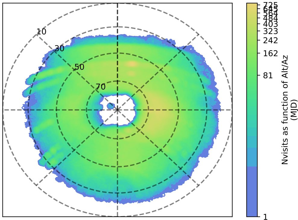
extra_ss_neo4_v3.4_10yrs u: Nvisits as function of Alt/Az
