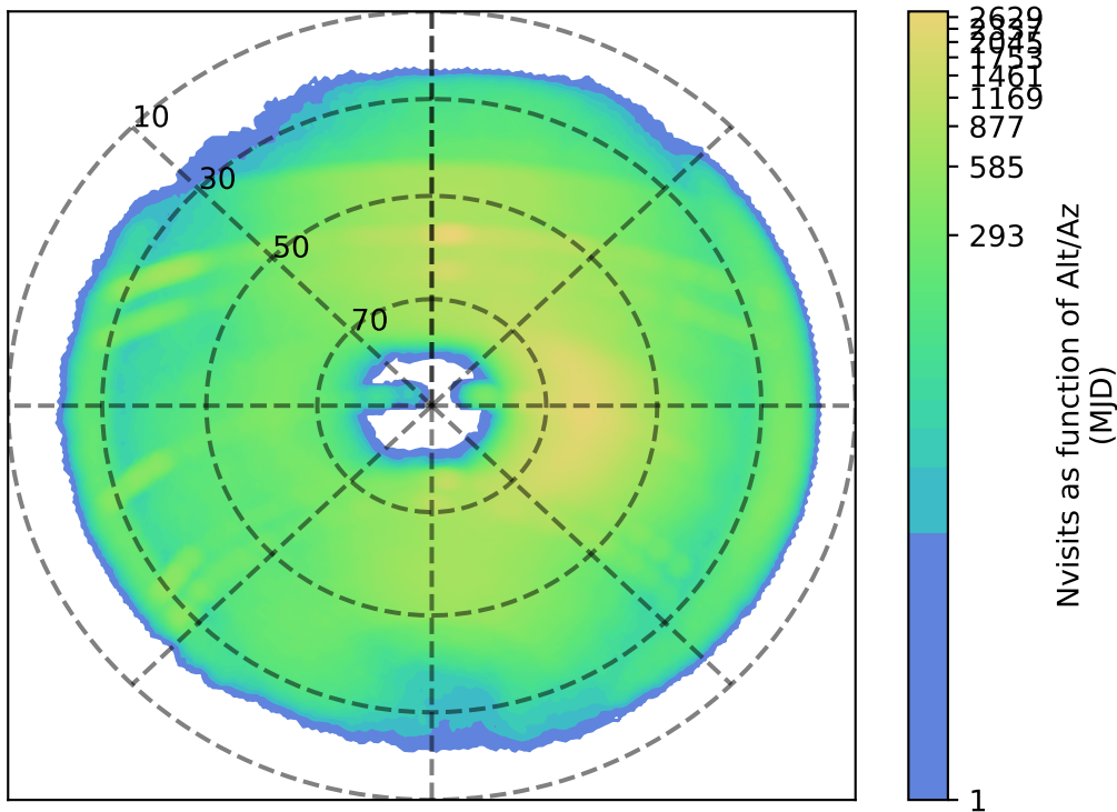
extra_ss_neo4_v3.4_10yrs i: Nvisits as function of Alt/Az
