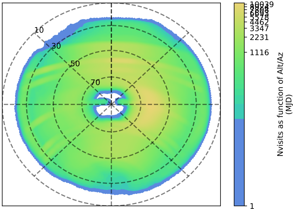
extra_ss_neo4_v3.4_10yrs : Nvisits as function of Alt/Az
