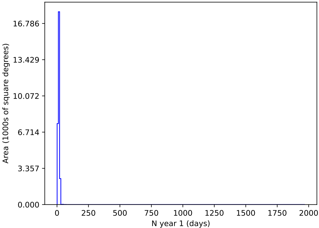
extra_ss_neo4_v3.4_10yrs z and night < 365: N year 1
