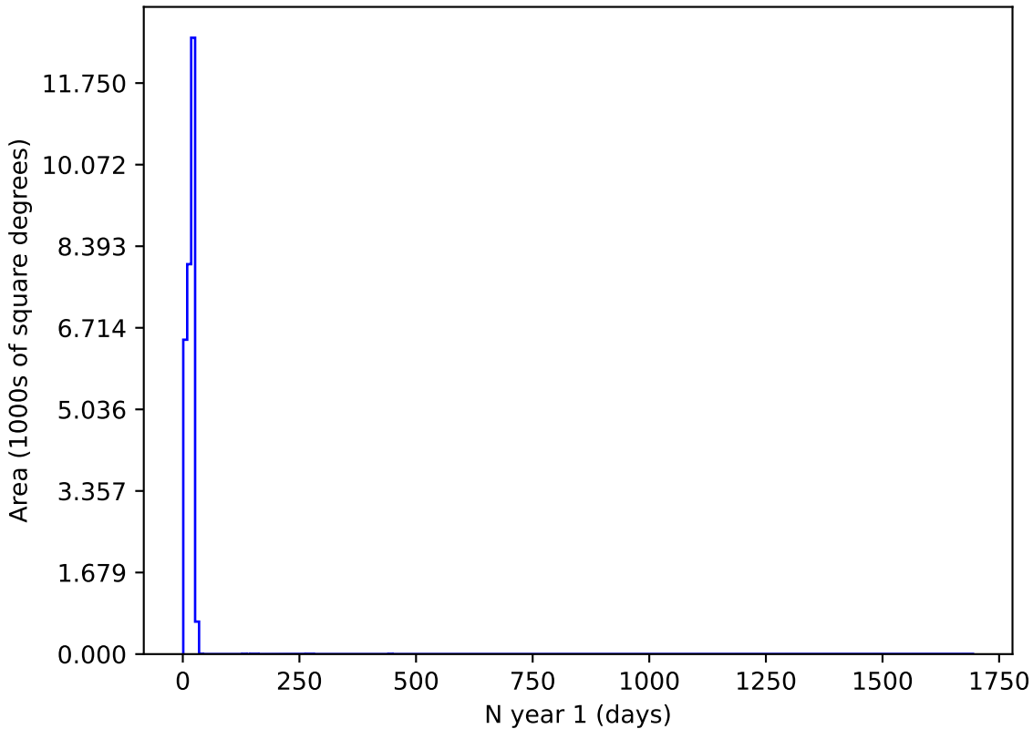
extra_ss_neo4_v3.4_10yrs r and night < 365: N year 1
