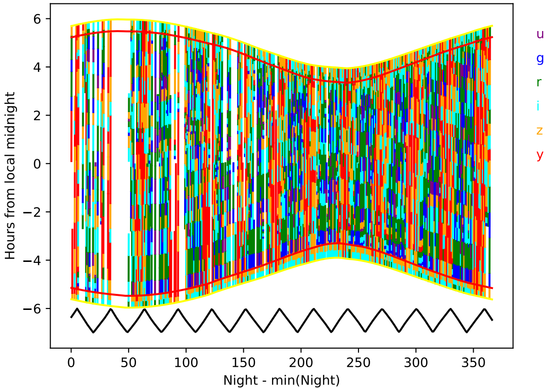
extra_ss_neo4_v3.4_10yrs year 6-7: Hourglass
