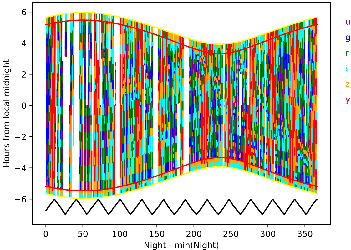
extra_ss_neo4_v3.4_10yrs year 0-1: Hourglass
