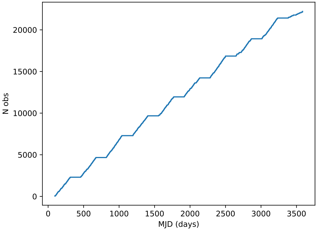
extra_ss_neo4_v3.4_10yrs note like DD:ECDFS%: Cumulative
