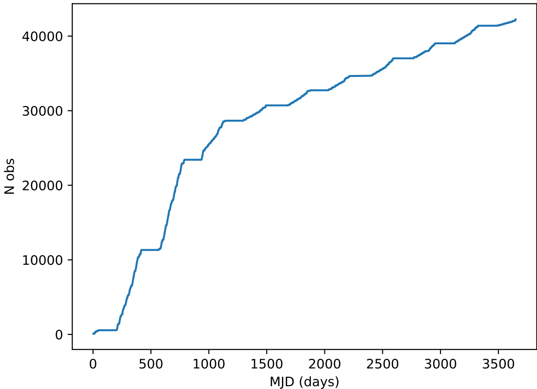
extra_ss_neo4_v3.4_10yrs note like DD:COSMOS%: Cumulative
