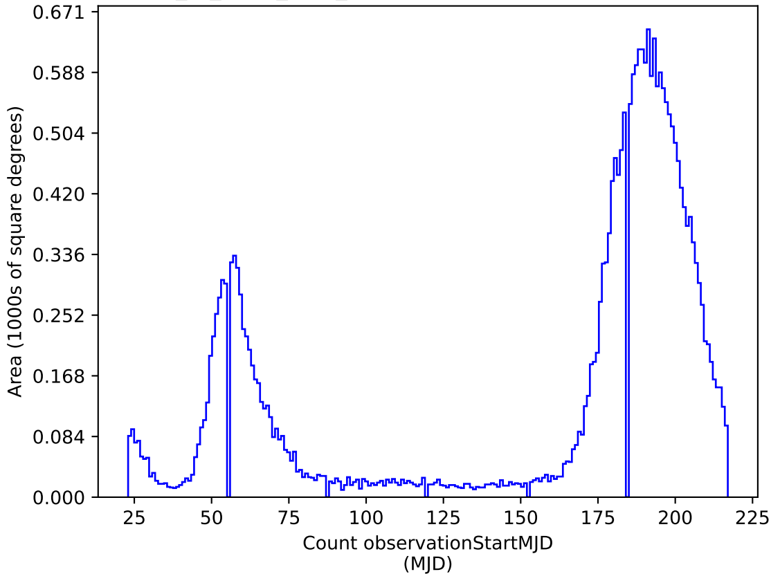
extra_ss_neo4_v3.4_10yrs i: Count observationStartMJD
