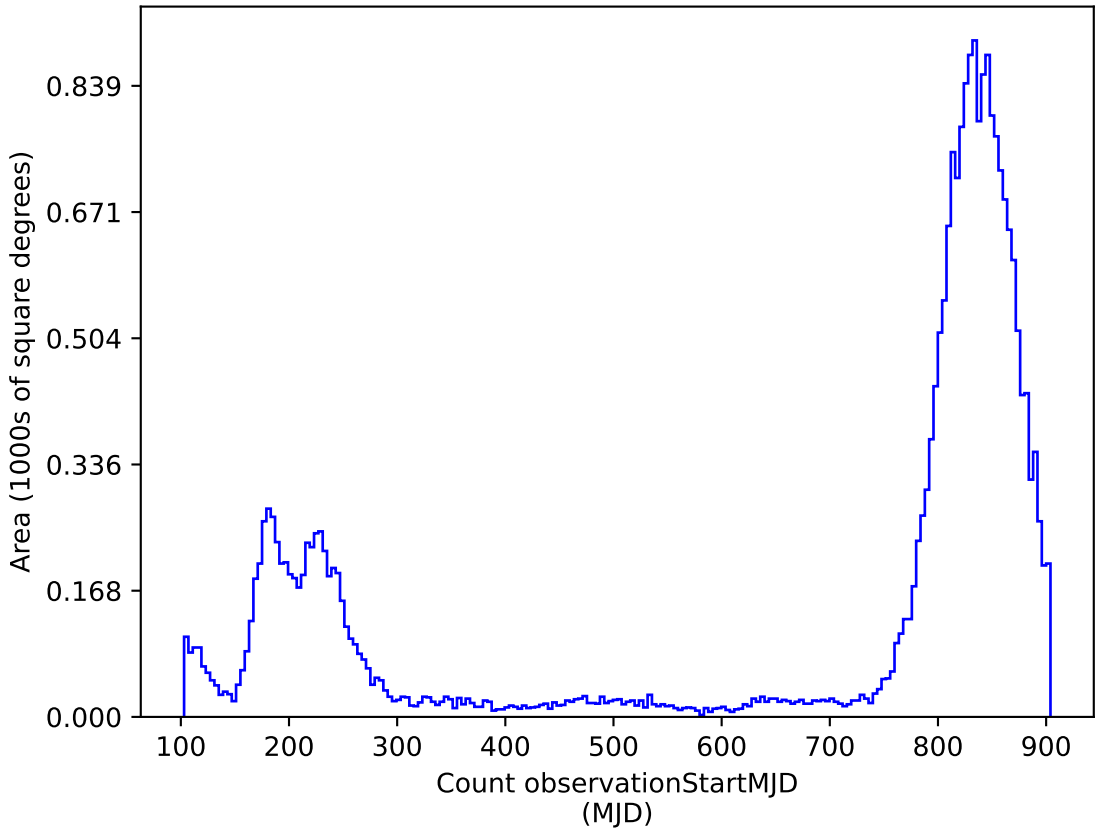
extra_ss_neo4_v3.4_10yrs : Count observationStartMJD
