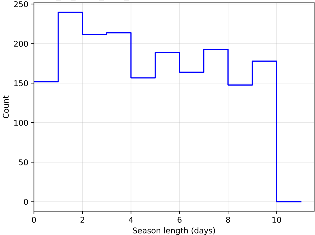
extra_ss_neo4_v3.4_10yrs DD:WFD all bands: SeasonLength
