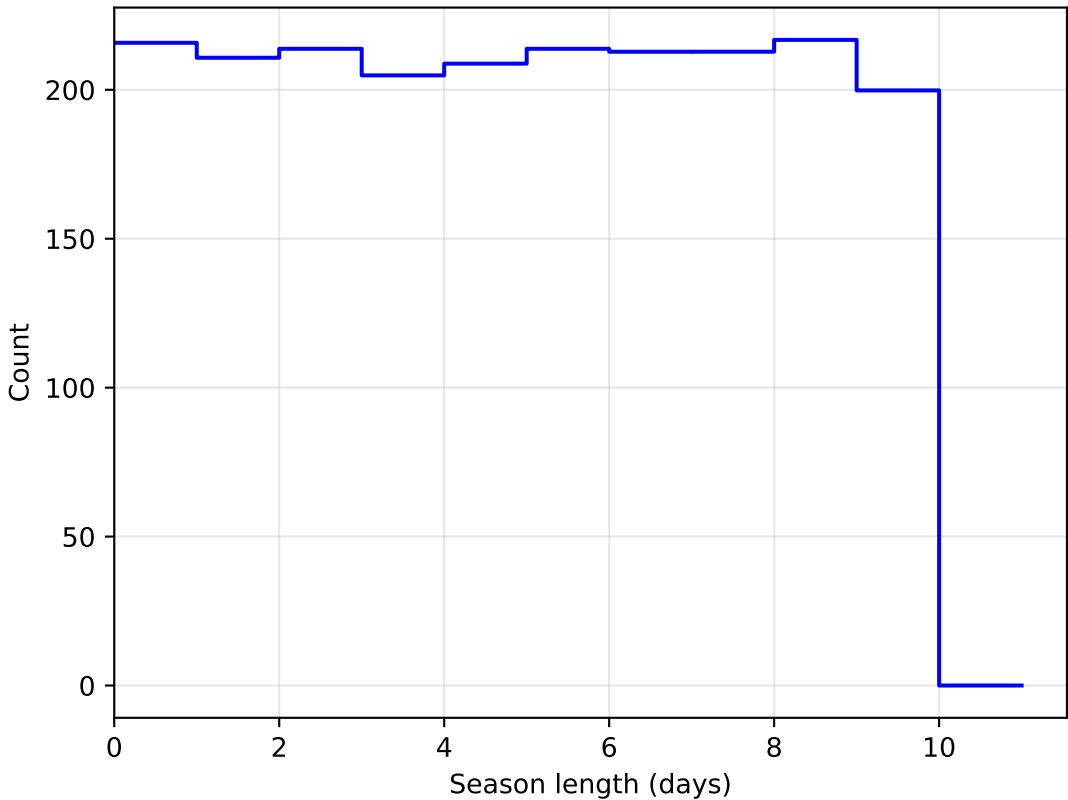
extra_ss_neo4_v3.4_10yrs DD:ECDFS all bands: SeasonLength
