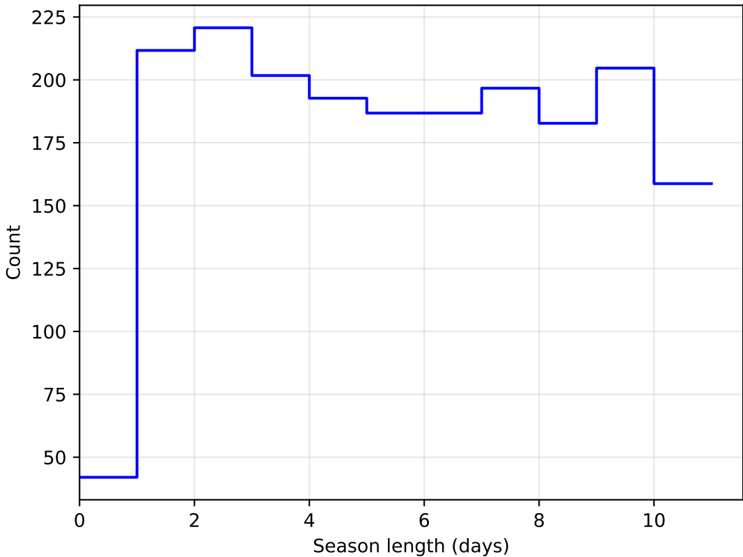
extra_ss_neo4_v3.4_10yrs DD: COSMOS all bands: SeasonLength
