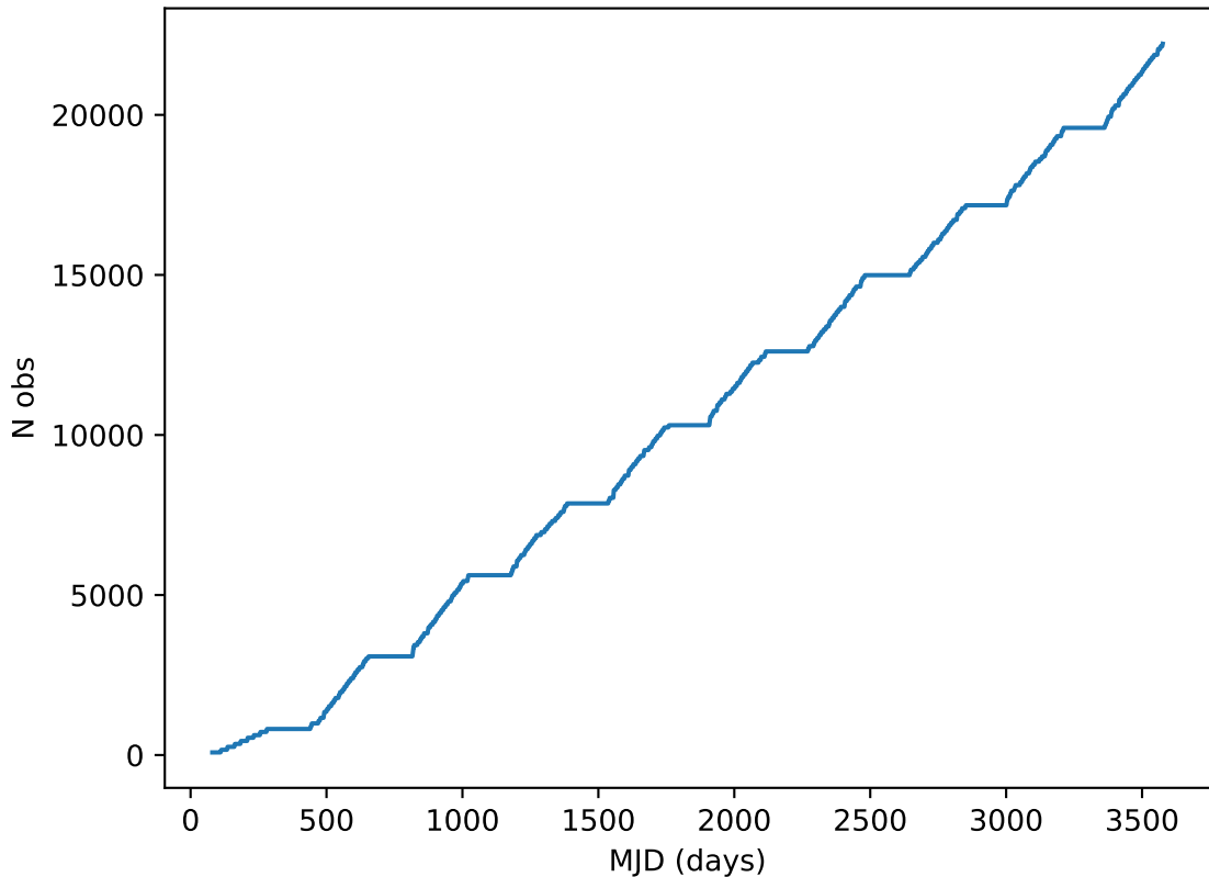
extra_ss_neo4_v3.4_10yrs all bands: DD:XMM_LSS Cumulative NVisits
