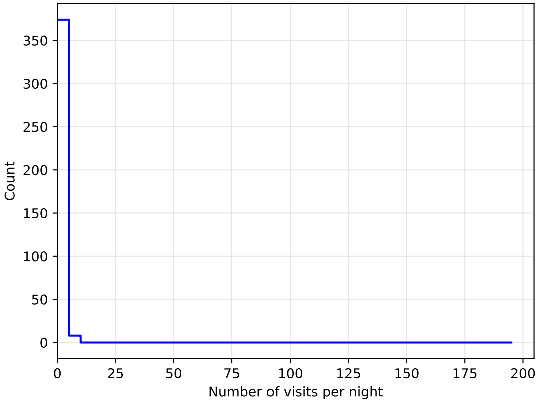
extra_ss_neo4_v3.4_10yrs all bands: DD:WFD NVisitsPerNight
