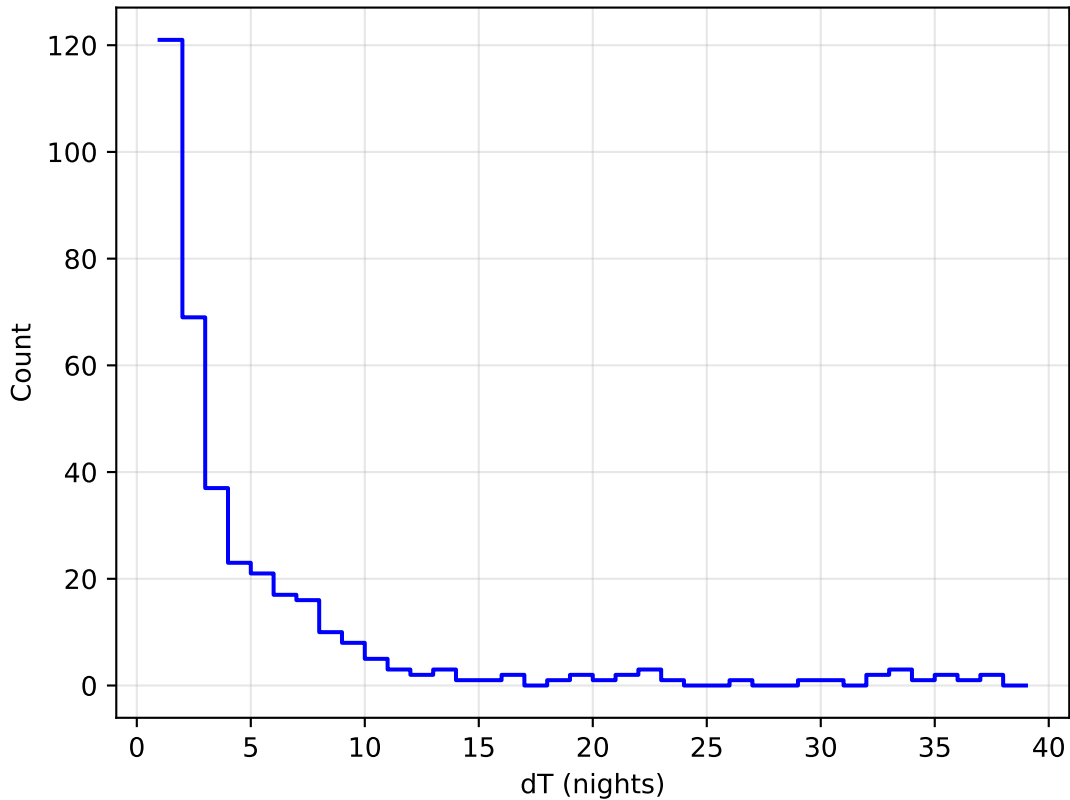
extra_ss_neo4_v3.4_10yrs all bands: DD:WFD Delta Nights Histogram
