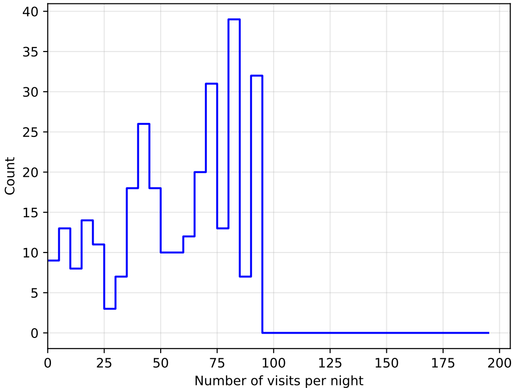
extra_ss_neo4_v3.4_10yrs all bands: DD:EDFS NVisitsPerNight
