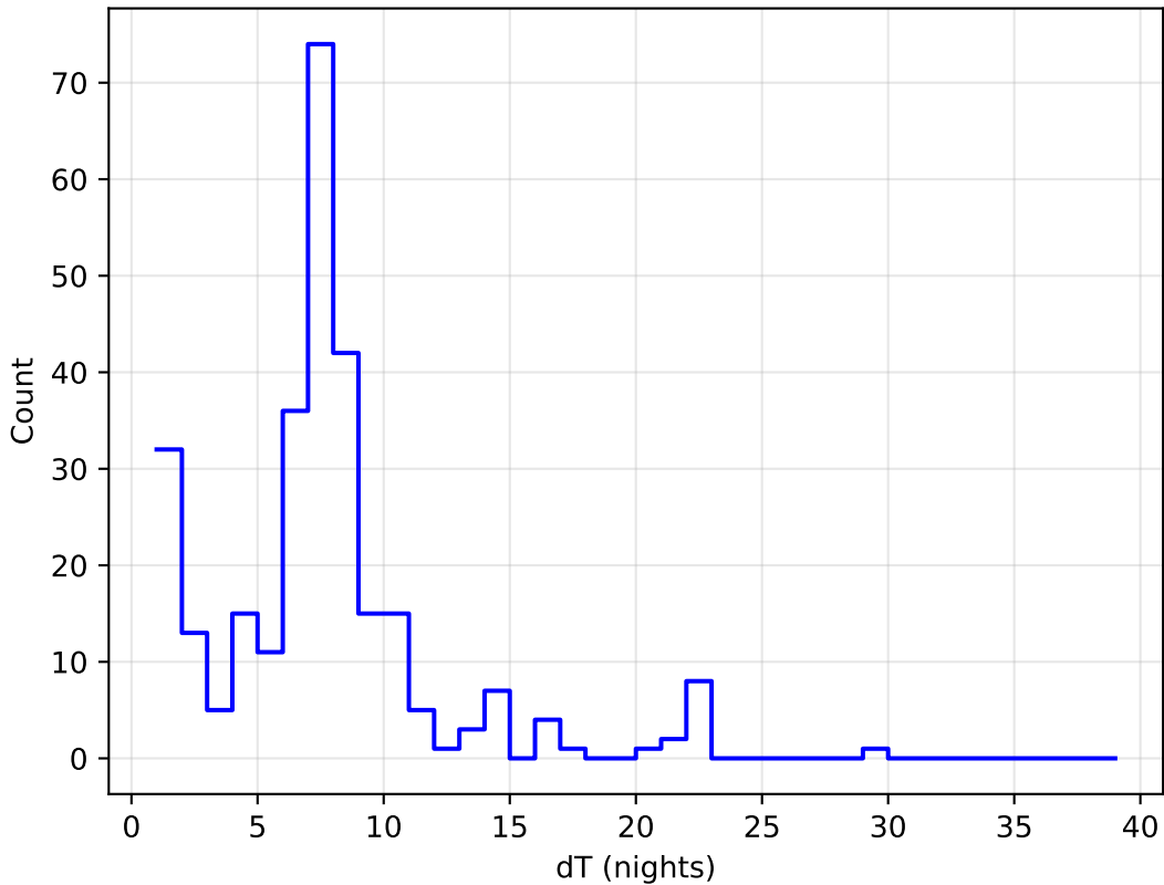
extra_ss_neo4_v3.4_10yrs all bands: DD:EDFS Delta Nights Histogram
