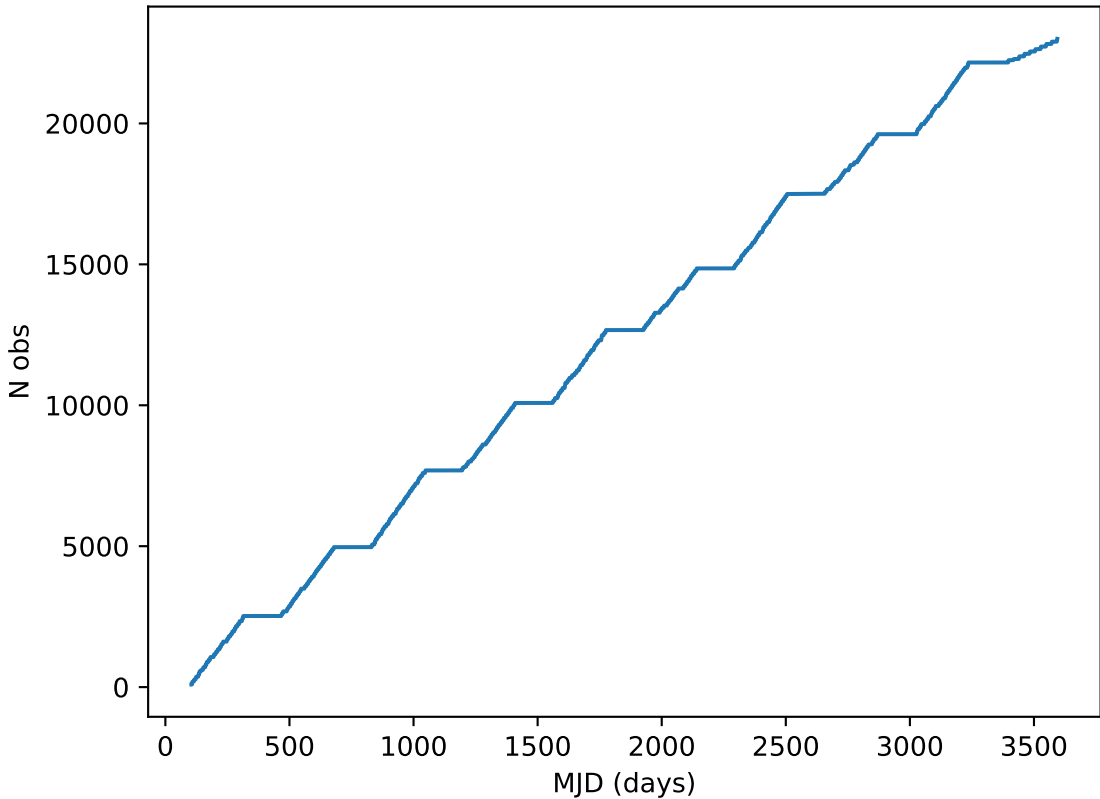
extra_ss_neo4_v3.4_10yrs all bands: DD:EDFS Cumulative NVisits
