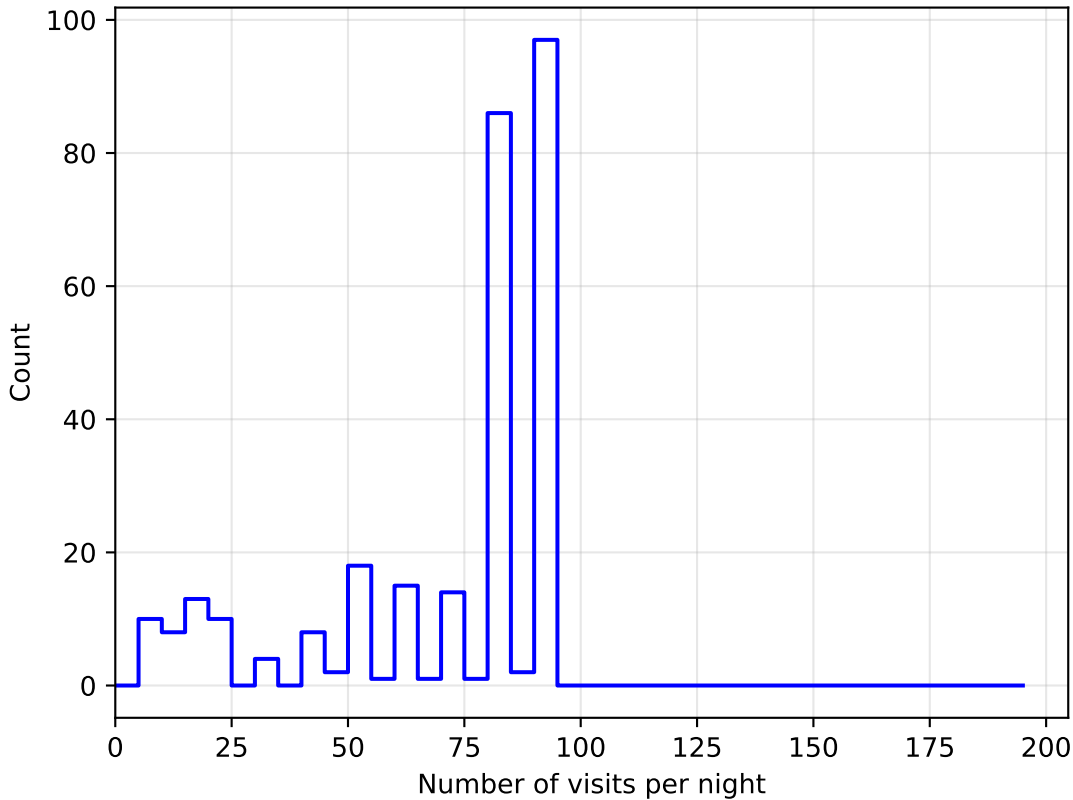
extra_ss_neo4_v3.4_10yrs all bands: DD:ECDFS NVisitsPerNight
