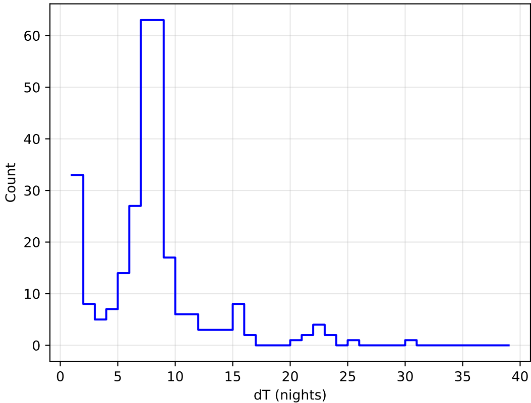
extra_ss_neo4_v3.4_10yrs all bands: DD:ECDFS Delta Nights Histogram
