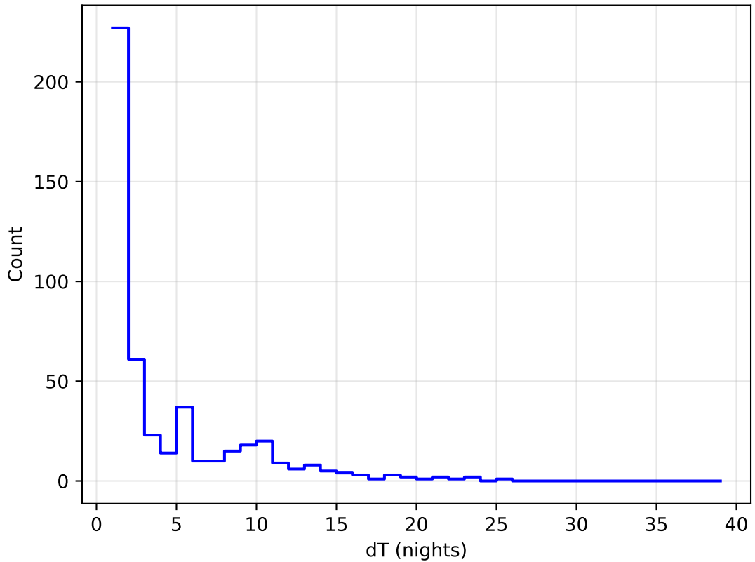
extra_ss_neo4_v3.4_10yrs all bands: DD: COSMOS Delta Nights Histogram
