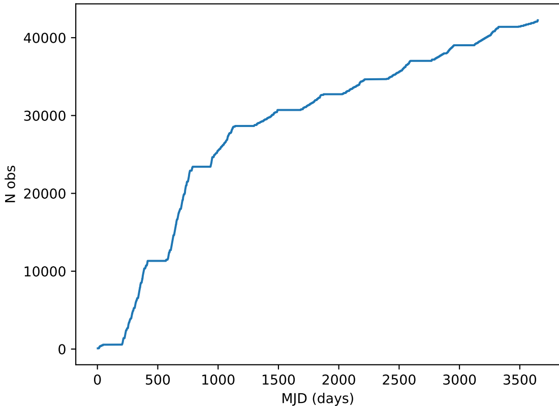
extra_ss_neo4_v3.4_10yrs all bands: DD:COSMOS Cumulative NVisits
