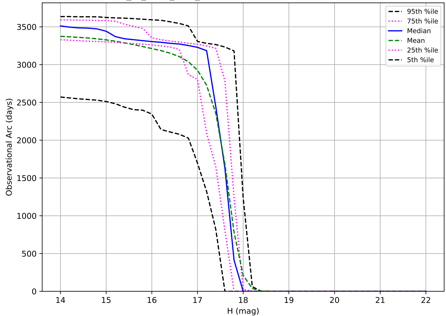
extra_ss_neo3_v3.4_10yrs: Observational Arc Length Trojan
