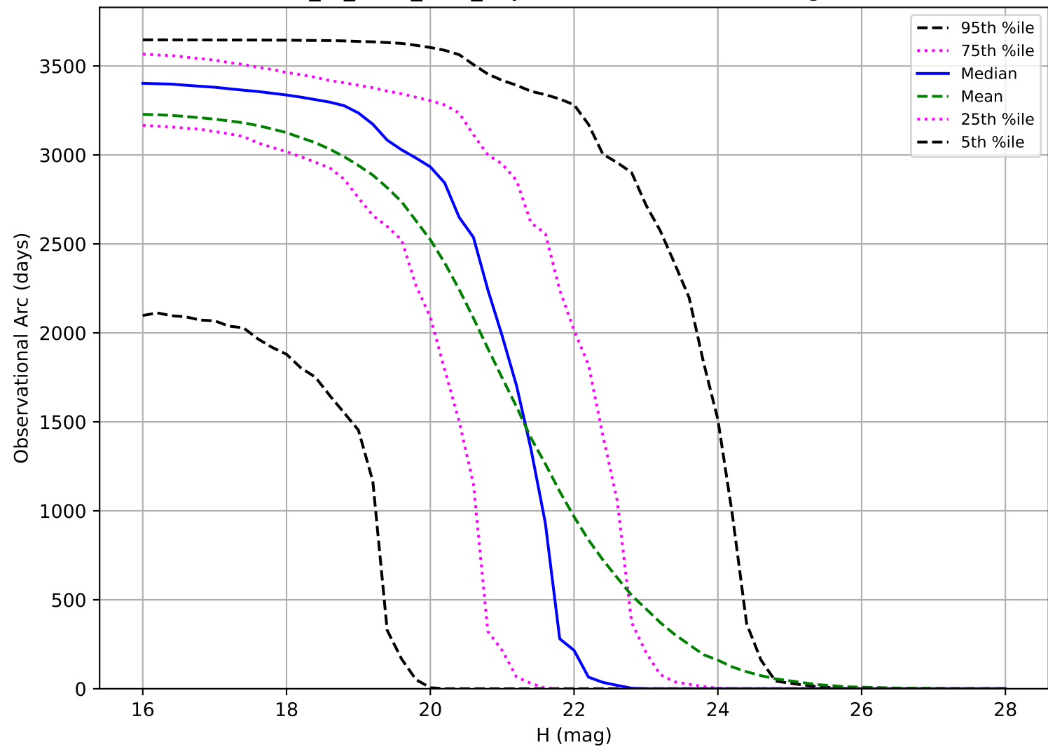
extra_ss_neo3_v3.4_10yrs: Observational Arc Length PHA
