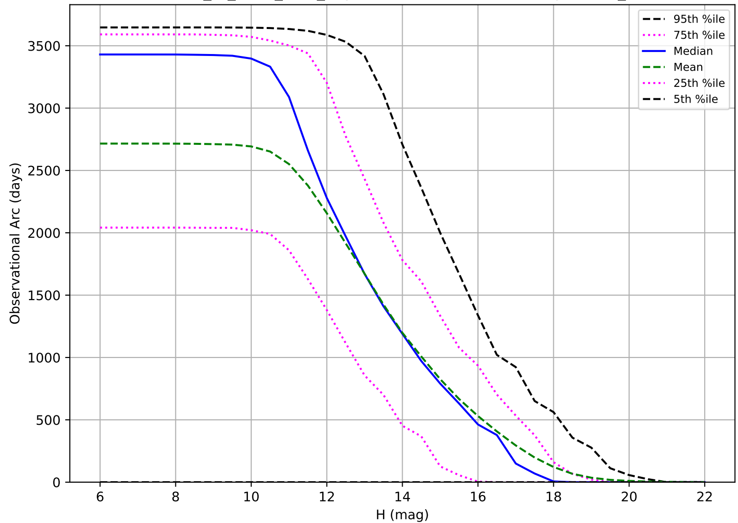
extra_ss_neo3_v3.4_10yrs: Observational Arc Length OCC_r5
