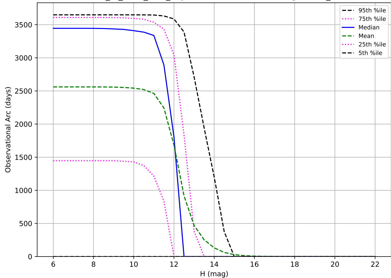
extra_ss_neo3_v3.4_10yrs: Observational Arc Length OCC_r20
