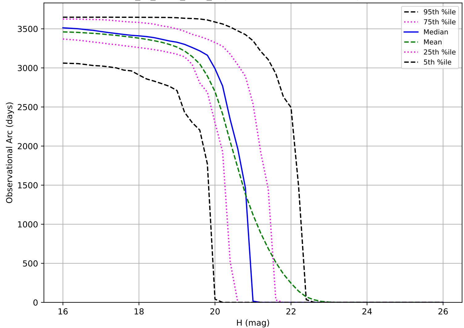
extra_ss_neo3_v3.4_10yrs: Observational Arc Length MBA
