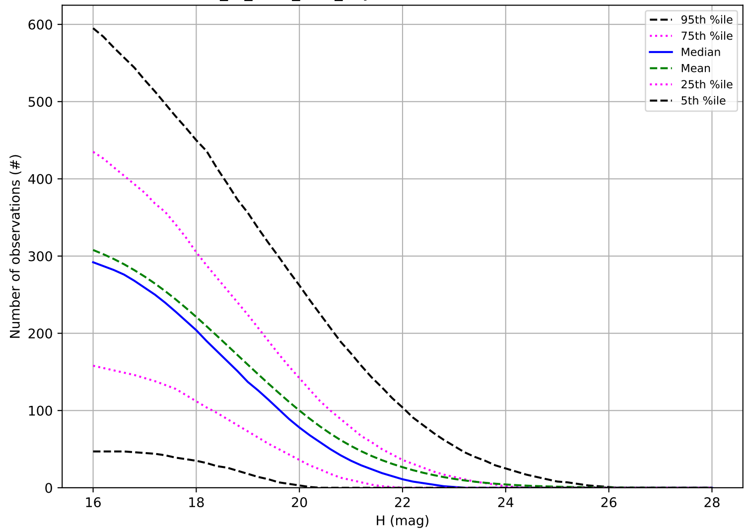
extra_ss_neo3_v3.4_10yrs: Number of observations PHA
