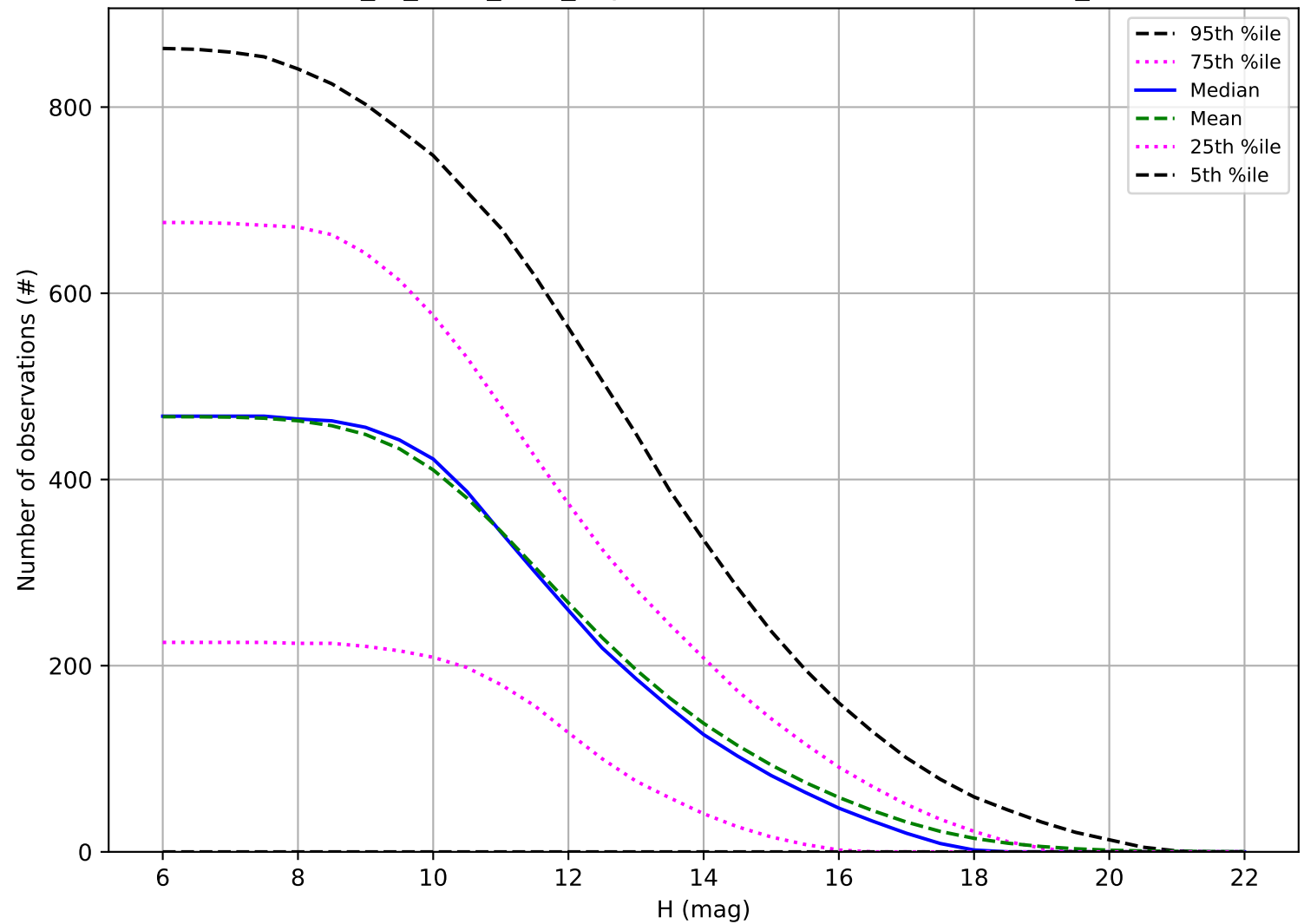
extra_ss_neo3_v3.4_10yrs: Number of observations OCC_r5
