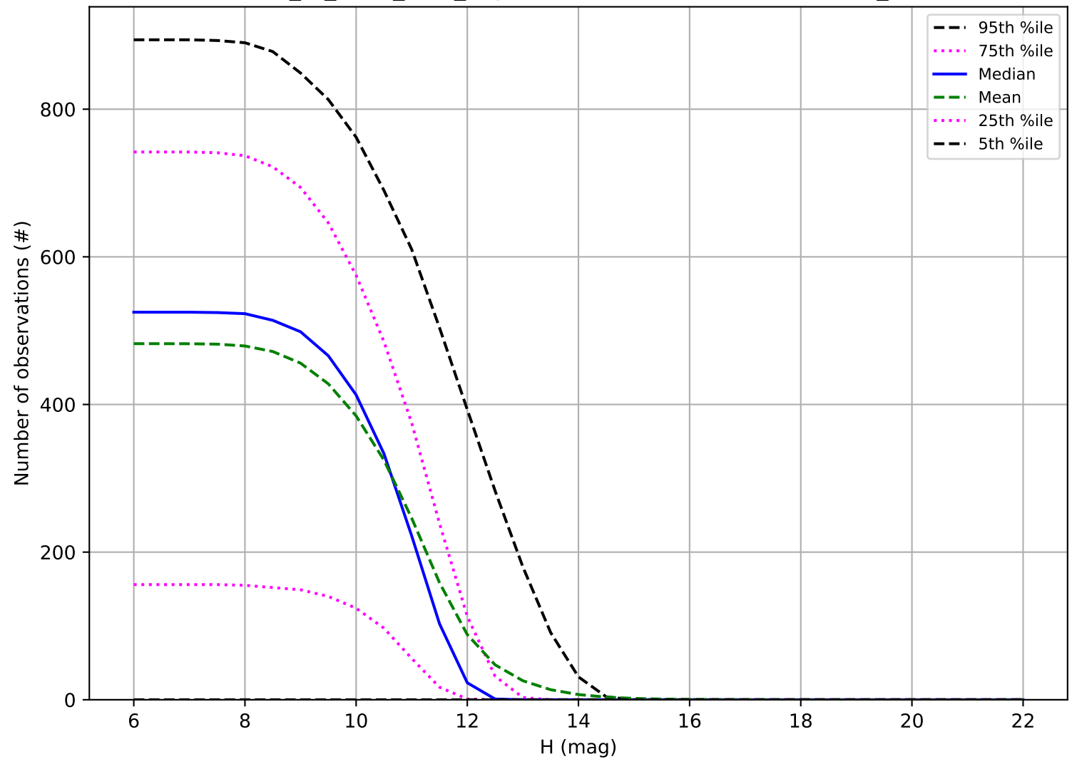
extra_ss_neo3_v3.4_10yrs: Number of observations OCC_r20
