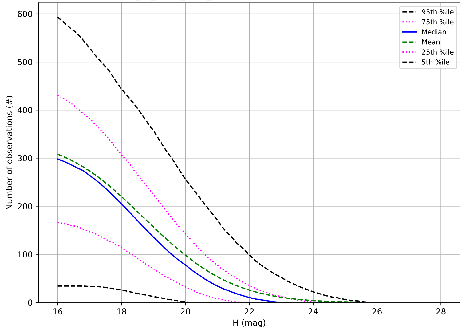
extra_ss_neo3_v3.4_10yrs: Number of observations NEO
