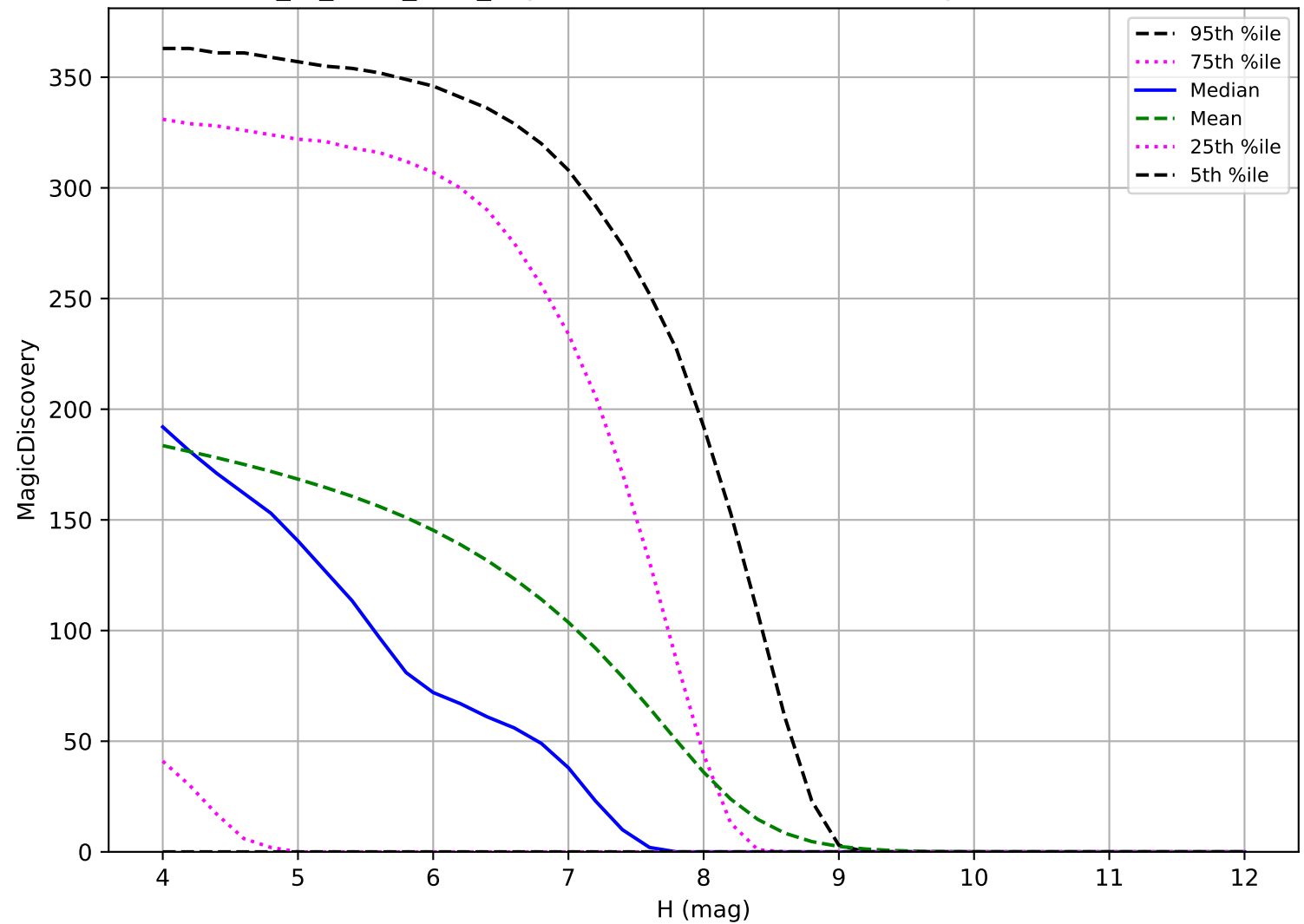
extra_ss_neo3_v3.4_10yrs: TNO 6 detections in 60 nights detection loss
