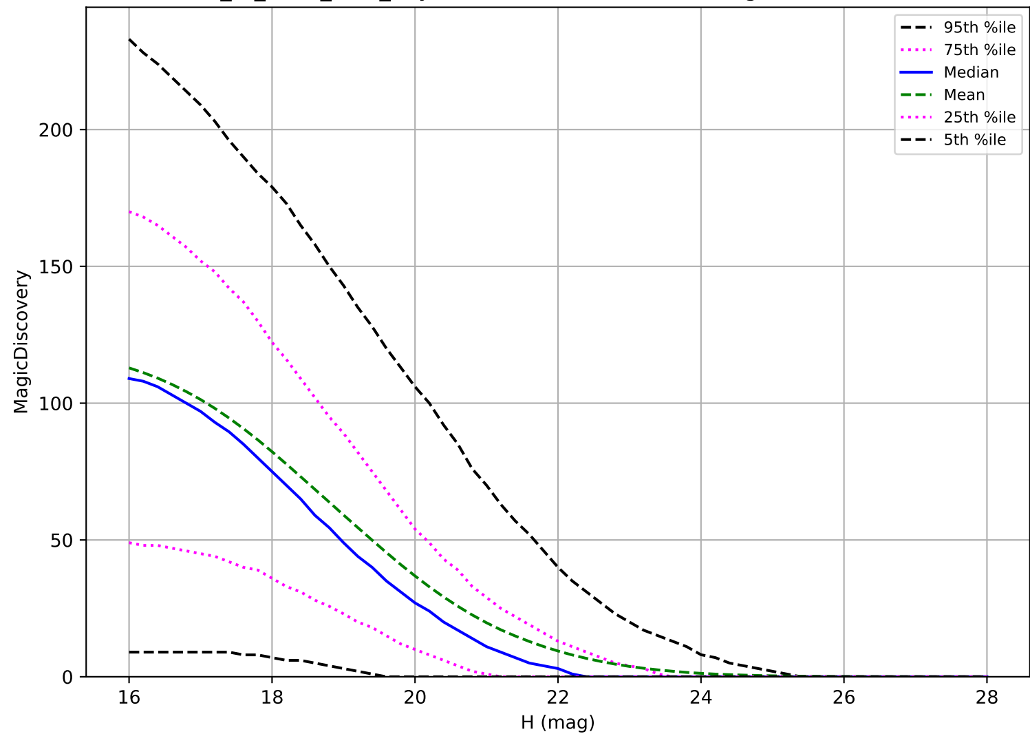
extra_ss_neo3_v3.4_10yrs: PHA 6 detections in 60 nights detection loss
