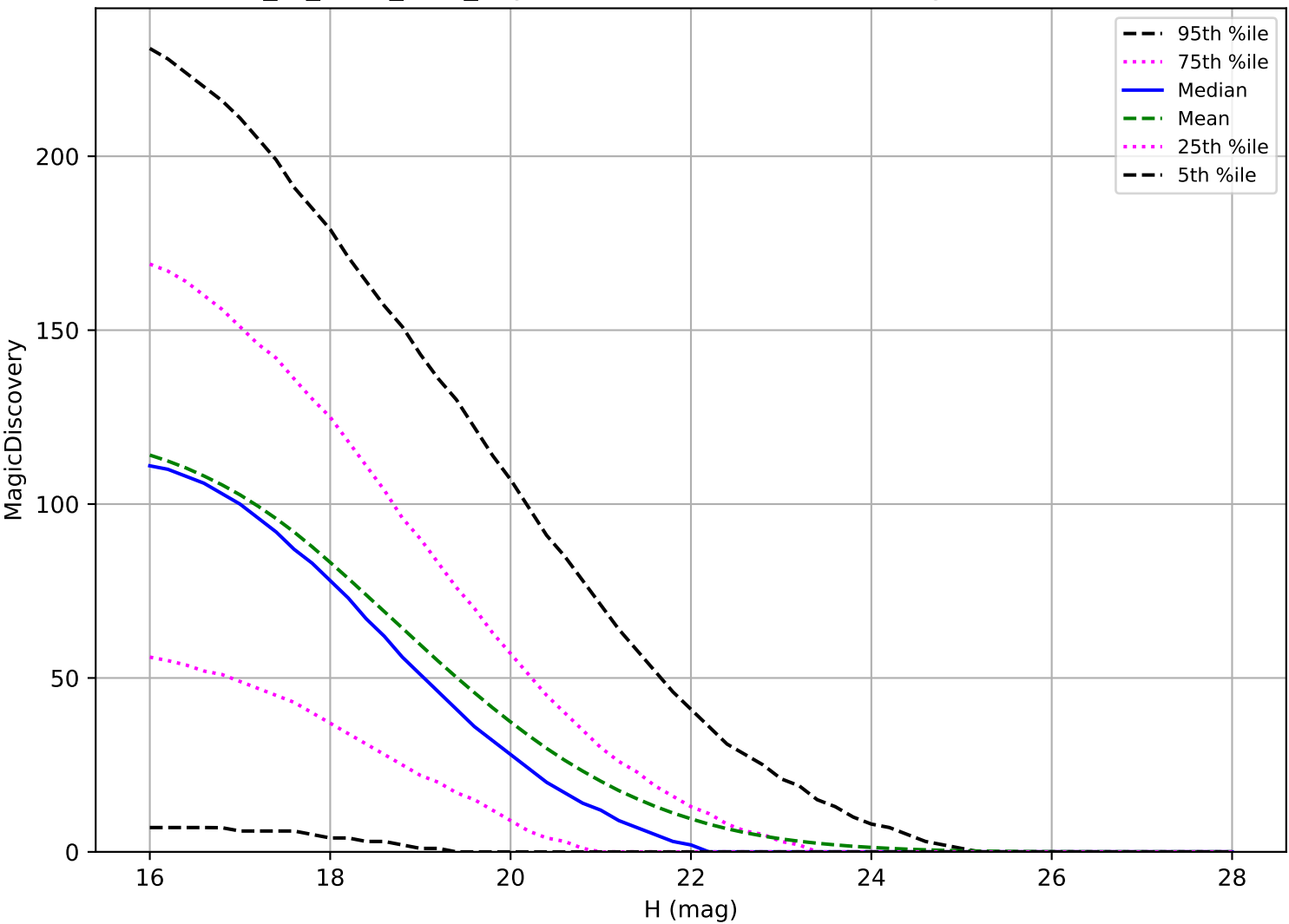
extra_ss_neo3_v3.4_10yrs: NEO 6 detections in 60 nights detection loss
