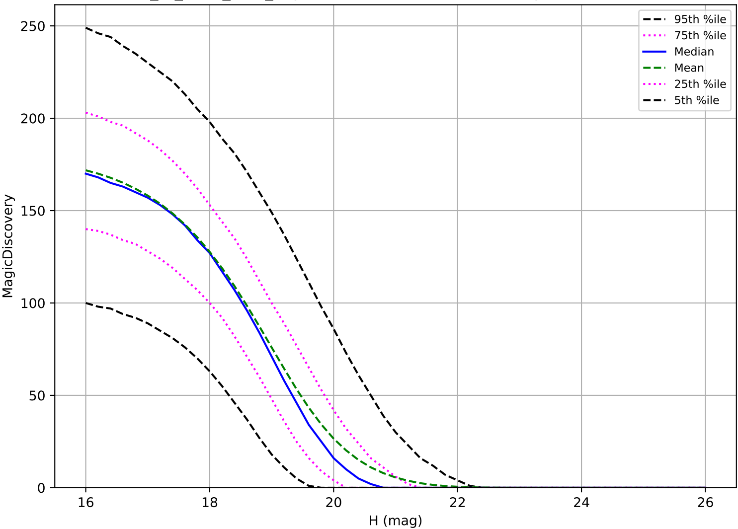
extra_ss_neo3_v3.4_10yrs: MBA 6 detections in 60 nights detection loss
