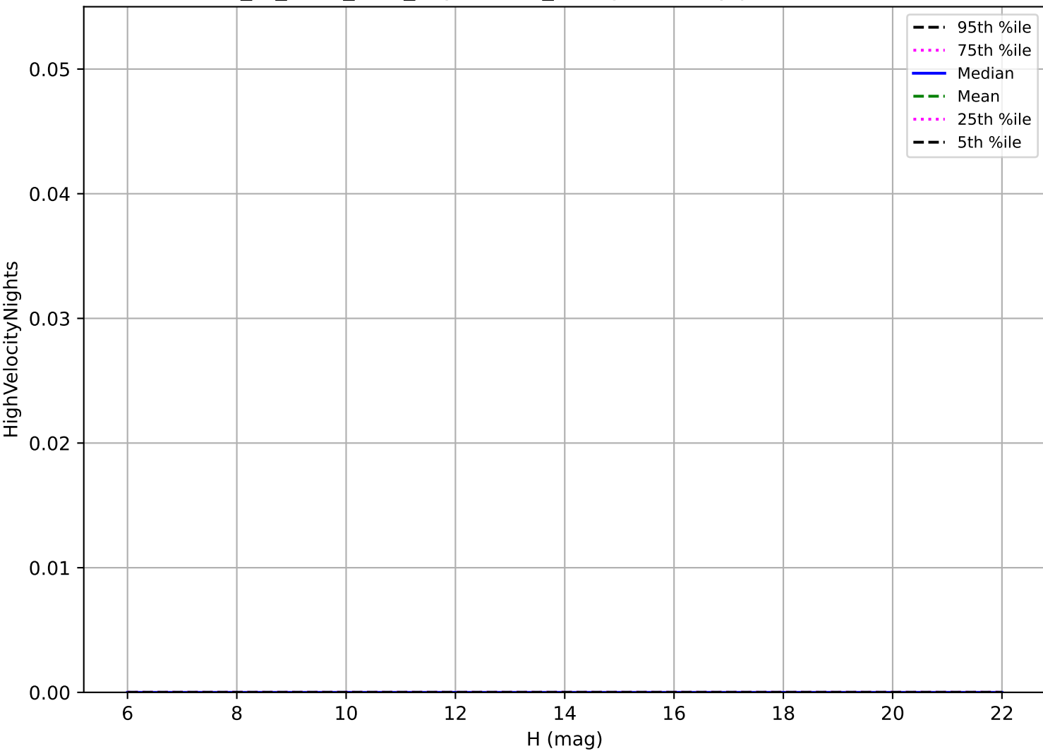
extra_ss_neo3_v3.4_10yrs: OCC_r5 High velocity pair detection loss
