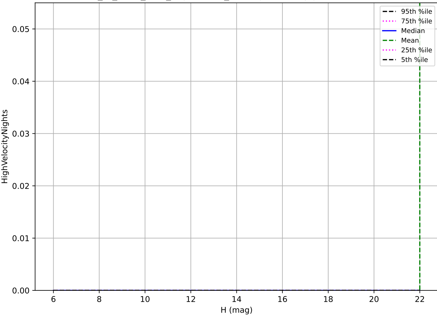
extra_ss_neo3_v3.4_10yrs: OCC_r20 High velocity pair detection loss
